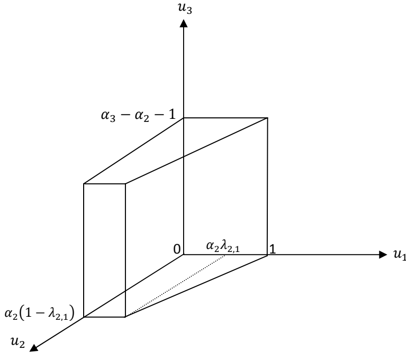
Figure 6: The bargaining set after agent two's manipulation.
