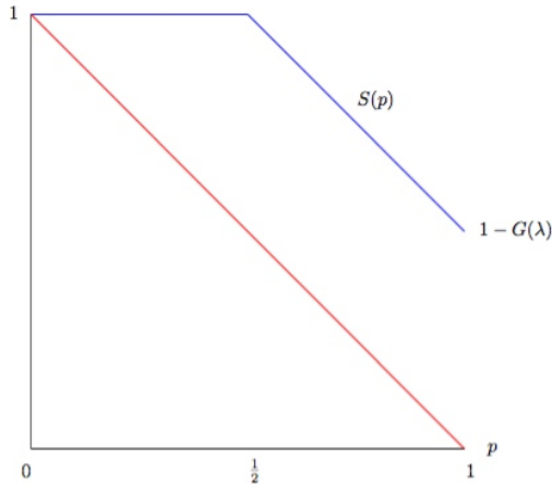
Figure 3: Illustration of Proposition 2. The blue curve represents S(p) , the ruler’s payoff with no media freedom, and the red line represents the ruler’s payoff from allowing complete media freedom. Parameters: \lambda = 1/2 .
